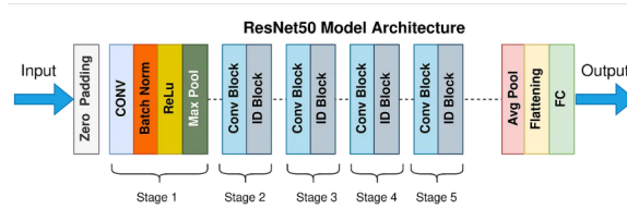
FIGURE 3. ResNet-50 architecture used for lesion classification.
